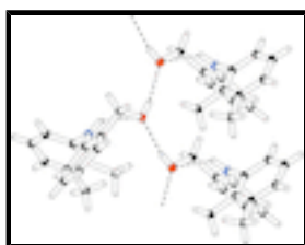
Fig. 3. The partial packing ( PLATON ; Spek, 2009) showing that molecules are interlinked and form supramolecular chains via O–H...O hydrogen bonding (dashed lines). The intramolecular S(6) ring motifs are also illustrated (dashed lines). Only the major component of the disordered group is shown for clarity.
