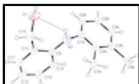
Fig. 2. View of (I) with the atom numbering scheme showing atoms of the minor component of the disorder. The displacement ellipsoids are drawn at the 50% probability level. H-atoms are shown as small spheres of arbitrary radii. The dotted line represent the intramolecular H-bonding.
